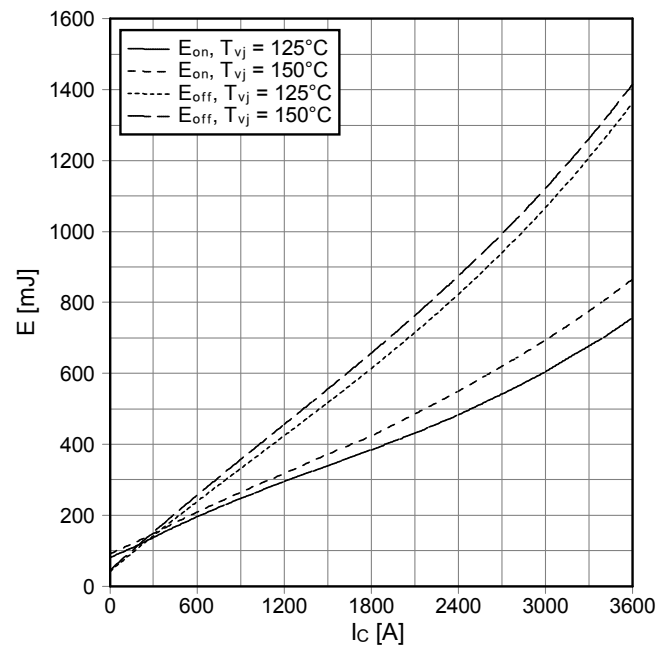
Schaltverluste IGBT-Wechselr. (typisch) switching losses IGBT-inverter (typical) E_{on} = f(I_c), E_{off} = f(I_c) V_{GE} = \pm 15\text{ V}, R_{Gon} = 0.5\ \Omega, R_{Goff} = 0.8\ \Omega, V_{CE} = 900\text{ V}
