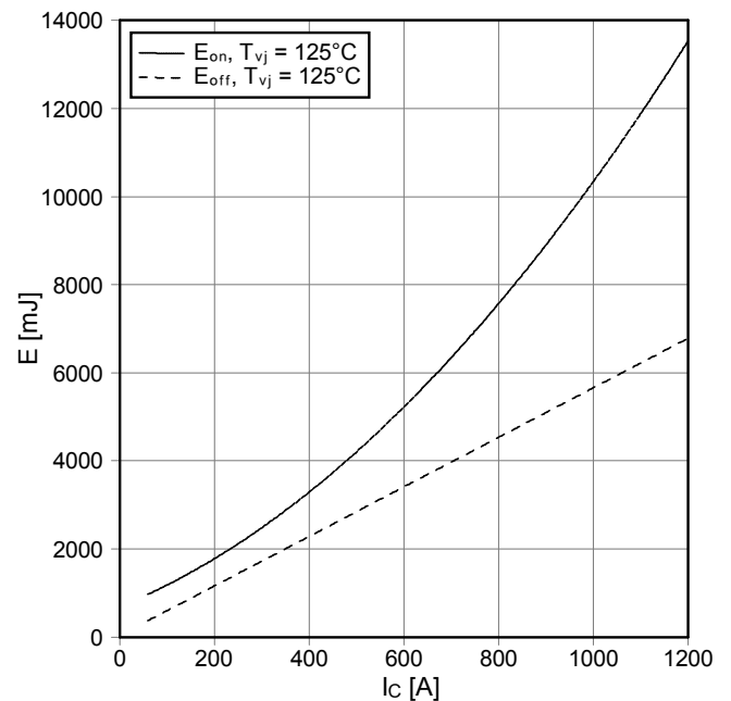
Schaltverluste IGBT-Wechselr. (typisch) switching losses IGBT-inverter (typical) E_{on} = f(I_C) , E_{off} = f(I_C) V_{GE} = \pm 15\text{ V} , R_{Gon} = 1.3\ \Omega , R_{Goff} = 8.2\ \Omega , V_{CE} = 3600\text{ V}
