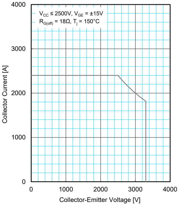
REVERSE BIAS SAFE OPERATING AREA (RBSOA)
